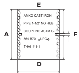
Pictured Below: 4" heavy-duty no hub gasket, cut-away view
