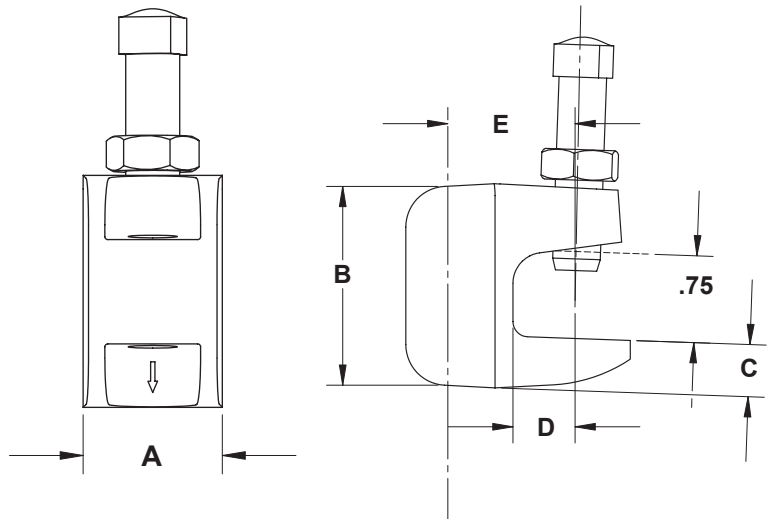
ELECTROPLATED BEAM CLAMPS | Dimensions [IN.]
