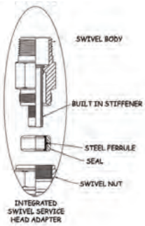
DETAIL VIEW TOP CONNECTION
