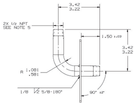
APPLIANCE STUB-OUT
