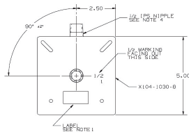
APPLIANCE STUB-OUT
