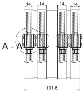
Pictured Below: 8" No-Hub band clamp detail
