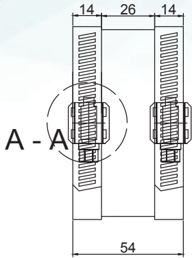
Pictured Below: 4" No-Hub band clamp detail
