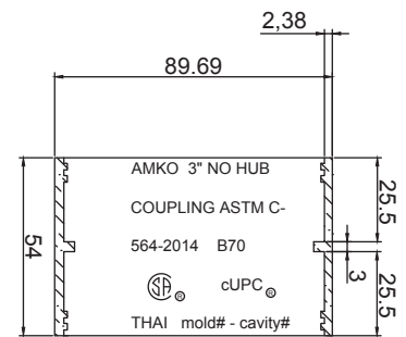
Pictured Below: 3" standard no-hub gasket, cut-away view
